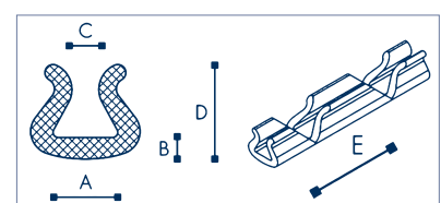
U-profil, multishape
